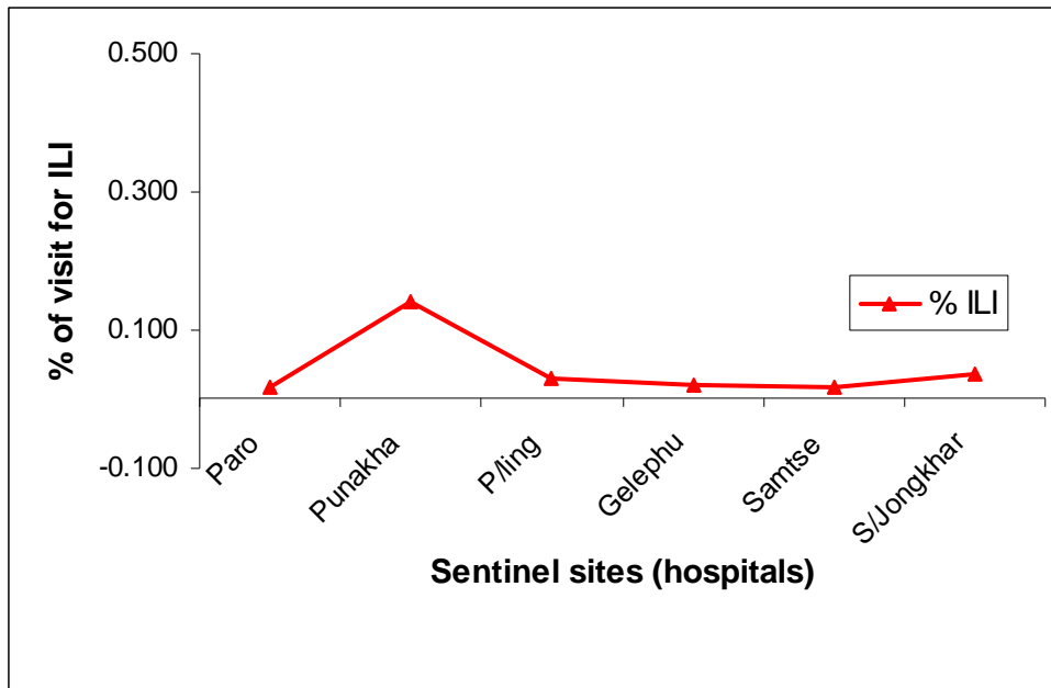
Figure 1: Percentage of Visits for Influenza-like Illness (ILI) reported by each sites
