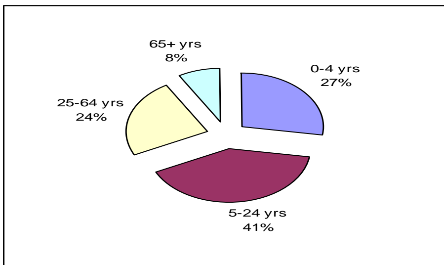
Figure 2: Age distribution among ILI cases
